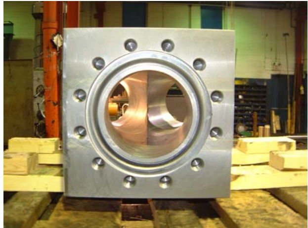
6" 900# A350 LF2 Wye with clamp pipe connectors
